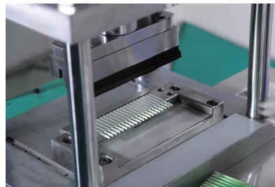
Swab Handle Final Cutting Process ( After Passing Inspection on Swab Head Quality Checking )
